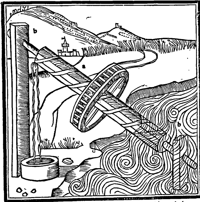
a. cocleæ ad rationem tri- goni pytha- gonicæ erectæ b. tigna in q̄ uersatur co- clea.
